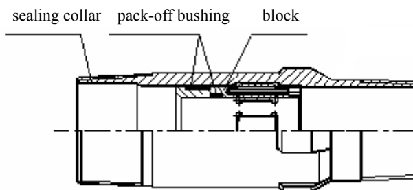
Fig. 4: Seal assembly
