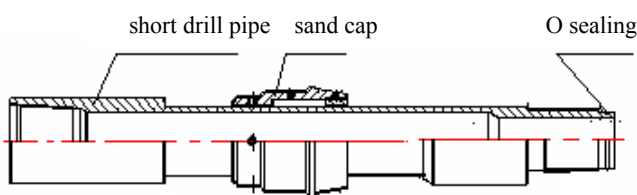
Fig. 2: Setting tool (A)
