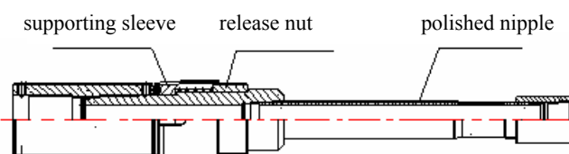
Fig. 3: Setting tool (B)
