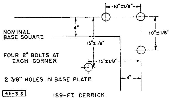
Figure B-3—Foundation Bolt Pattern for Derrick Leg
