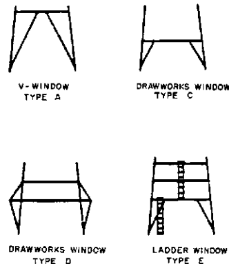
Figure B-2—Derrick Windows
