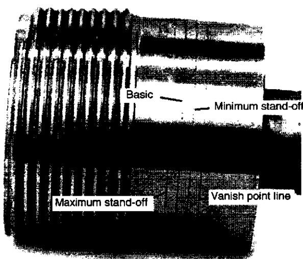
Figure 37—Standoff Lines Style Plug Gauge
