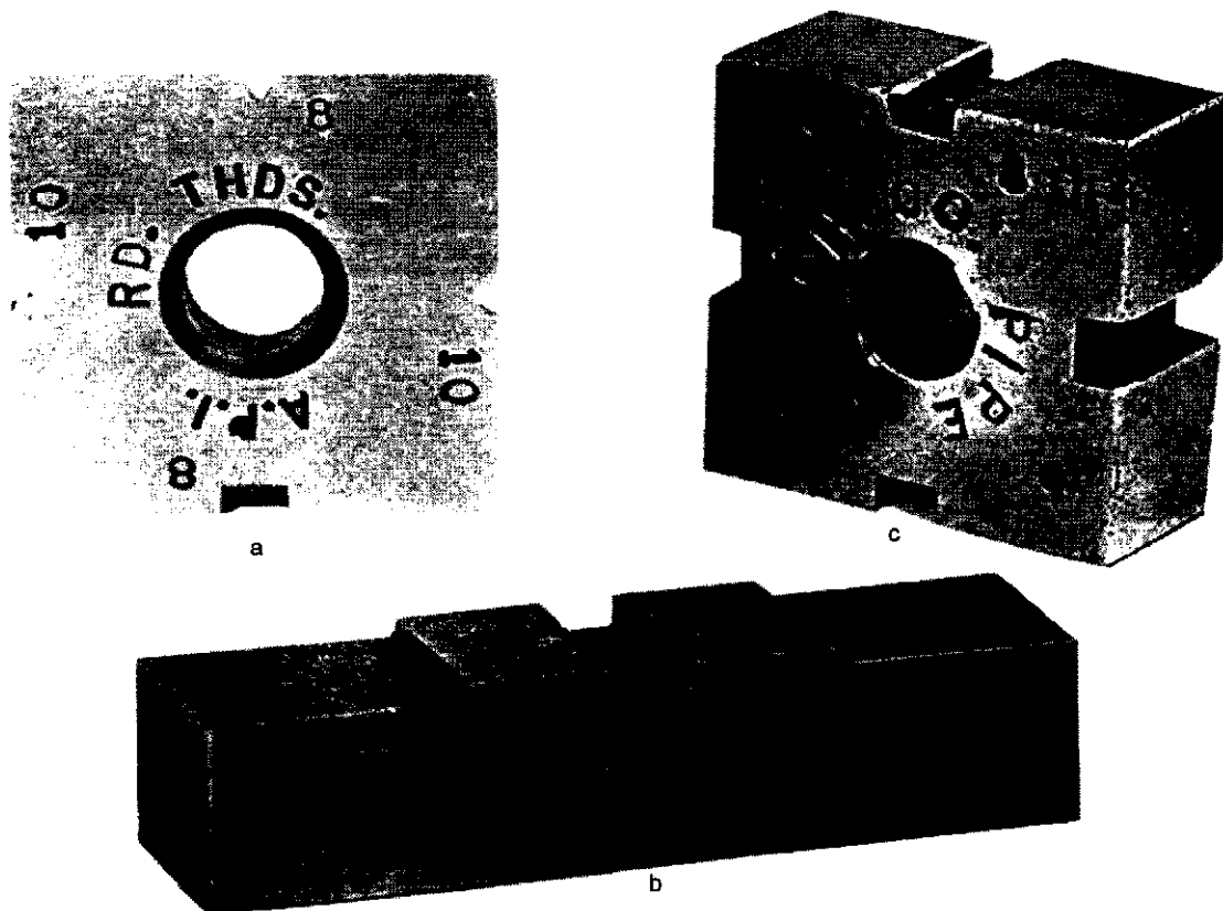
Figure 20—Setting Standards for (a) API Round and Vee-Type Threads, (b) Extreme-Line and 16-in. and Larger Buttress Threads, and (c) Vee-Block Setting Standard for Contact and Point Verification
