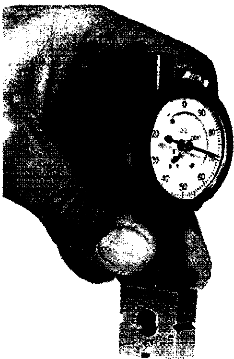
Figure 22—Continuous-Dial Height Gauge Applied to a Vee Block
