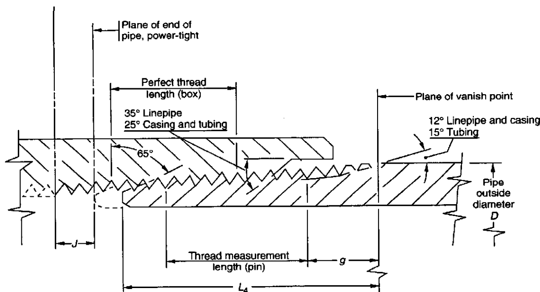
Figure 15—Basic Dimensions of Line Pipe Threads and Casing and Tubing Round Threads (Hand-Tight Makeup)
