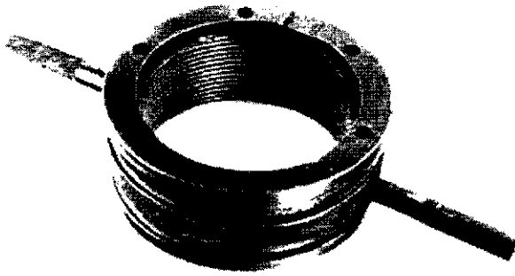
Figure 12—Fixed-Type Gauge
