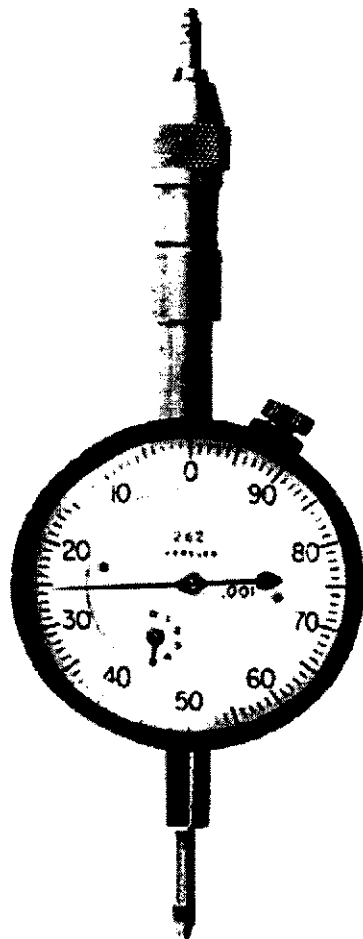
Figure 31—Assembled Internal Taper Gauge for 4½-in. OD and Larger Pipe
