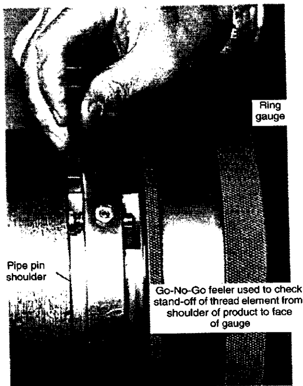
Figure 55—Extreme-Line Thread Ring Gauge Installed Hand-Tight and Seal Ring Advanced (Note use of Go-No-Go Gauge)
