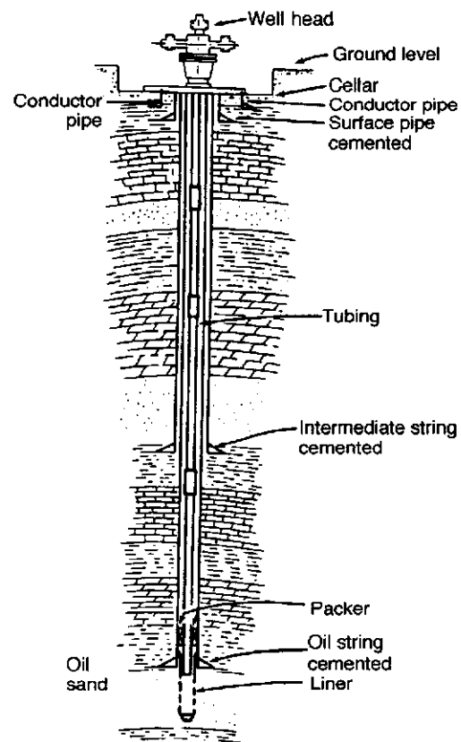
Figure 1—Schematic Diagram of an Oil or Gas Well Completed with a Hung Liner
