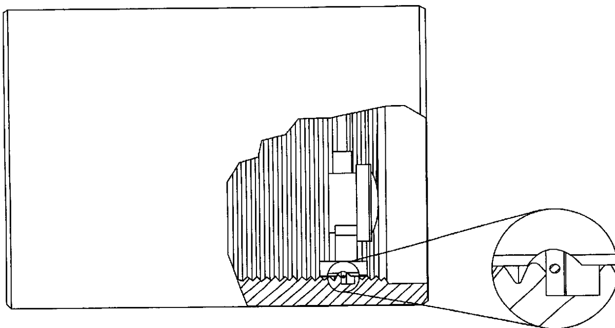
Figure 61—Gauging of Casing Coupling Grooves
