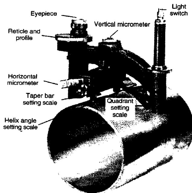
Figure 59—Thread Contour Microscope
