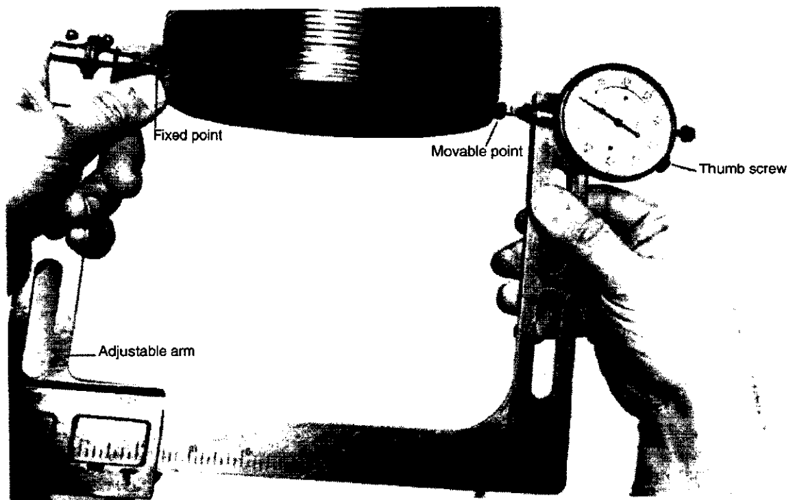
Figure 28—External Thread Taper Caliper
