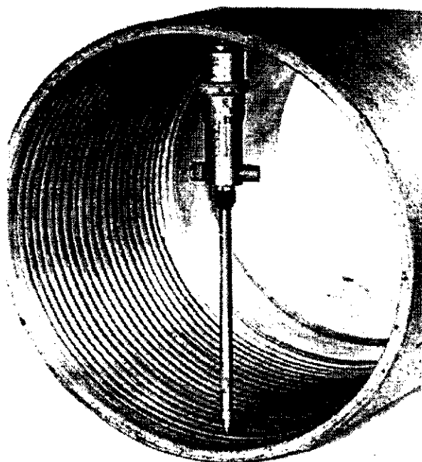
Figure 49—Internal Micrometer Fitted with Flat Contacts for Crest-to-Crest Measurement
