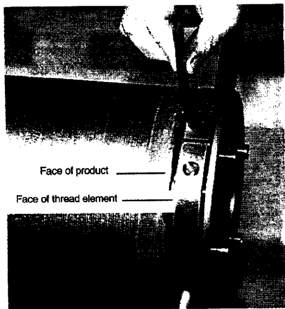
Figure 57—Extreme-Line Thread Plug Gauge Installed Hand-Tight and Seal Plug Advanced (Note use of Go-No-Go Gauge.)
