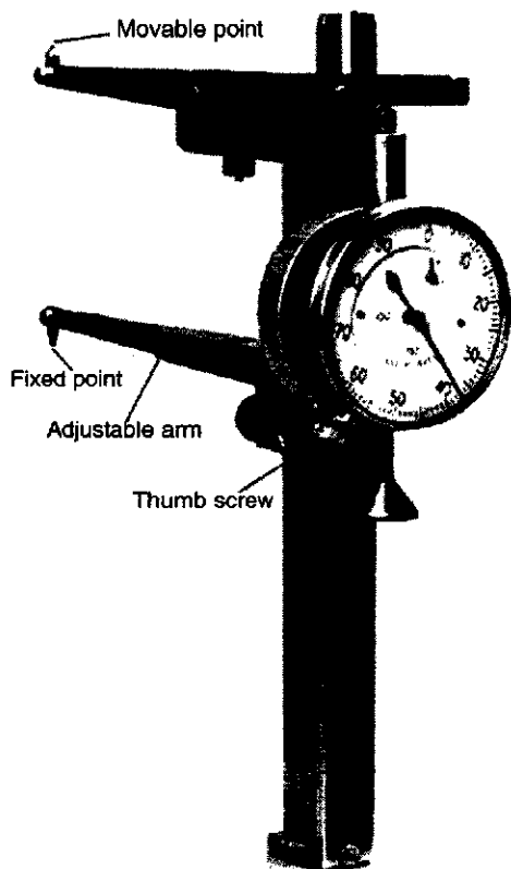
Figure 30—Internal Thread Taper Caliper for Pipe Less Than 4\frac{1}{2} -in. OD
