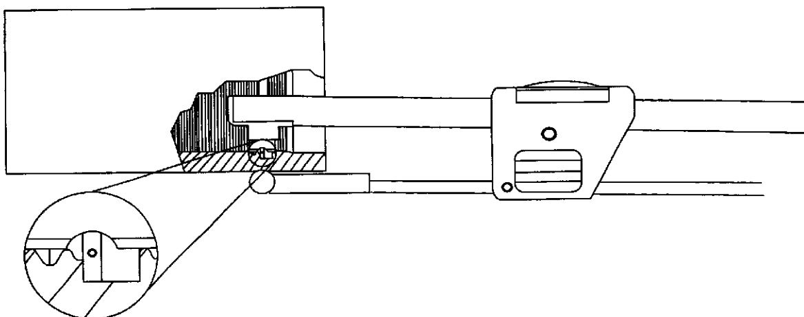
Figure 60—Gauging of Tubing Coupling Grooves
