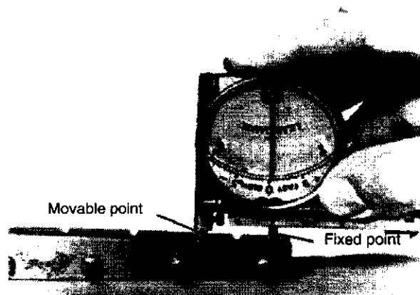
Figure 27—Lead Setting Standard with External/Internal Lead Gauge Applied
