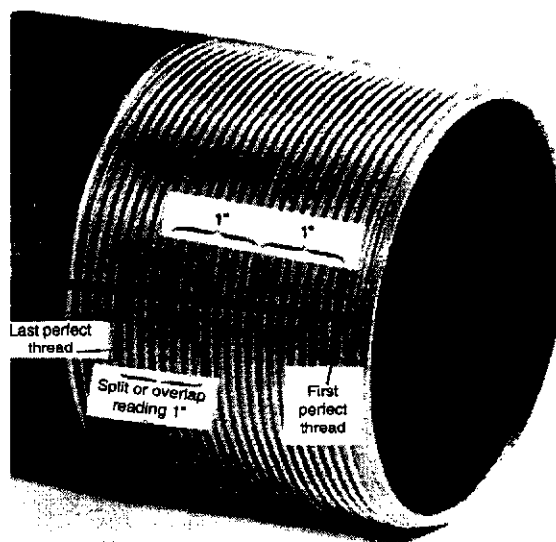
Figure 16—Pin End Thread on Which is Drawn a Longitudinal Line to Facilitate Inspection—Coupling Longitudinal Line is Drawn in Similar Manner
