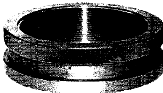
Figure 32—Flush-Type Ring Gauge
