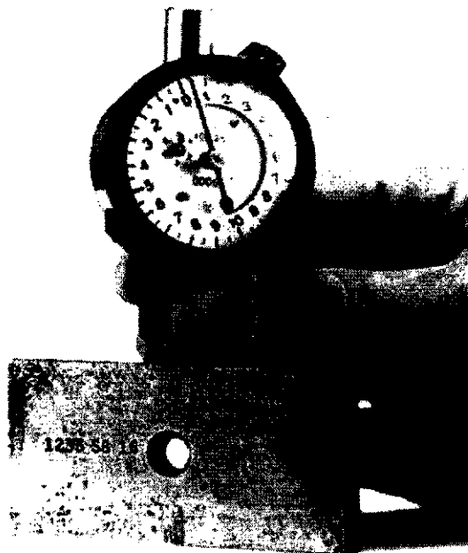
Figure 21—Height Gauge Applied to Setting Standard (Balanced-Type)
