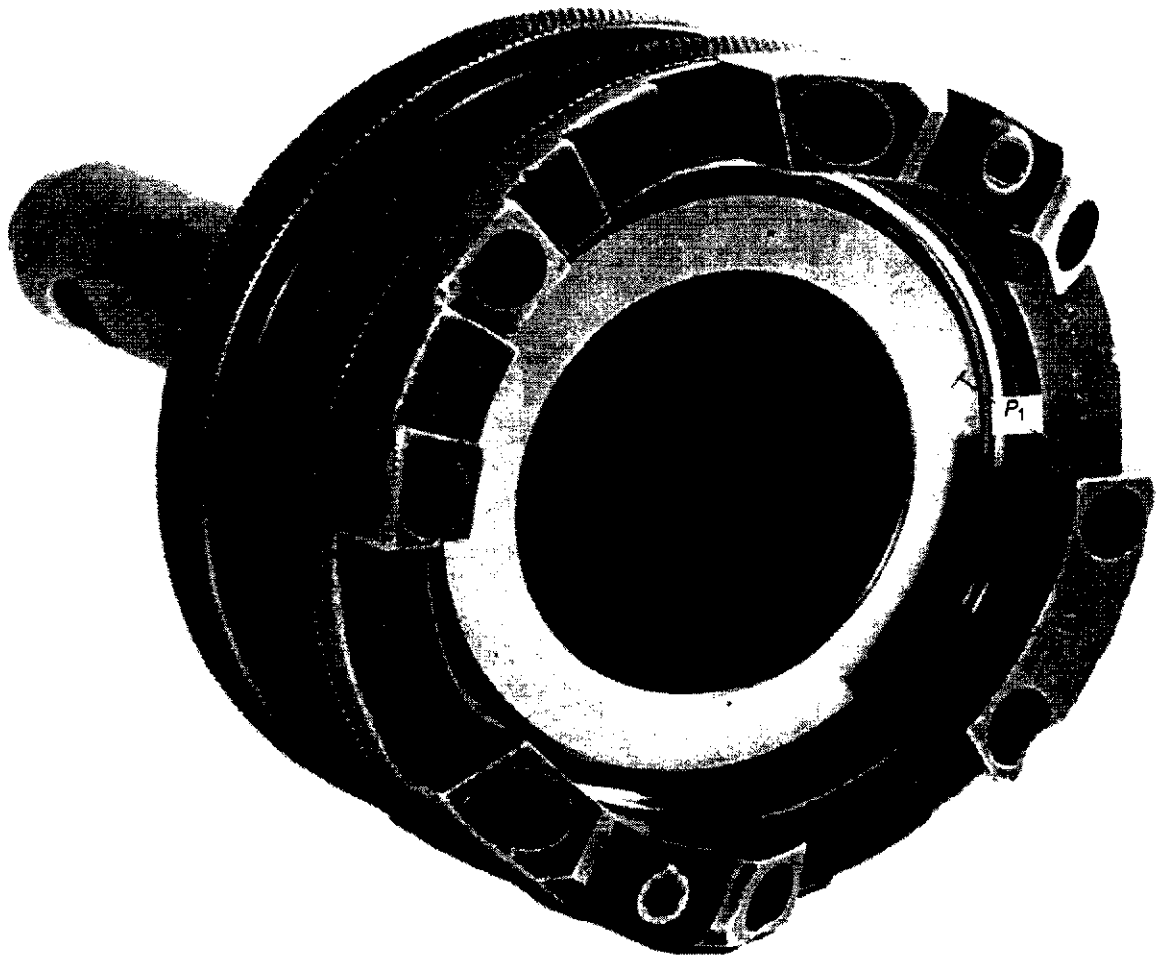
Figure 36—Standoff of Master Plug and Working Ring Gauges
