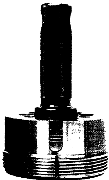
Figure 33—Insert Style Plug Gauge
