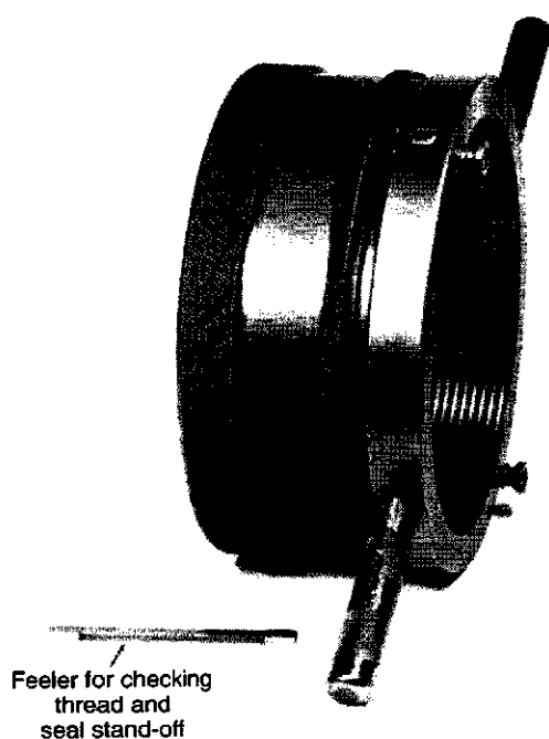
Figure 51—Extreme-Line Thread Ring Gauge with Sliding Seal Gauging Ring
