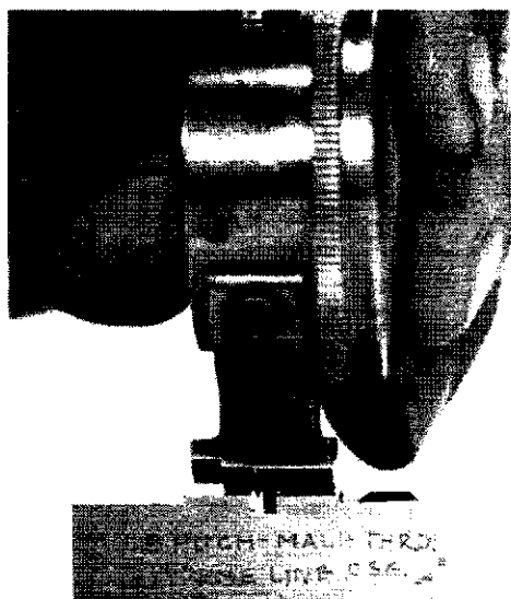
Figure 48—Extreme-Line Thread Height Gauge Setting Standard
