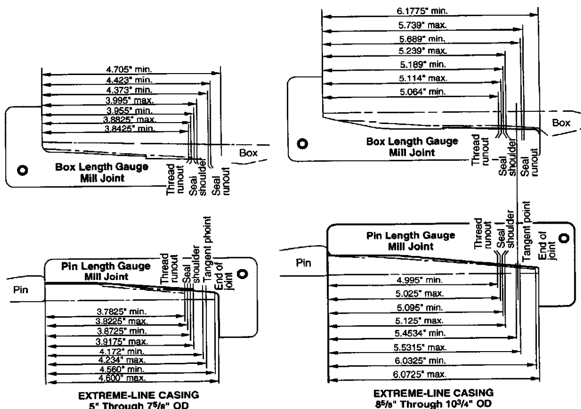
Figure 43—Extreme-Line Length Templates
