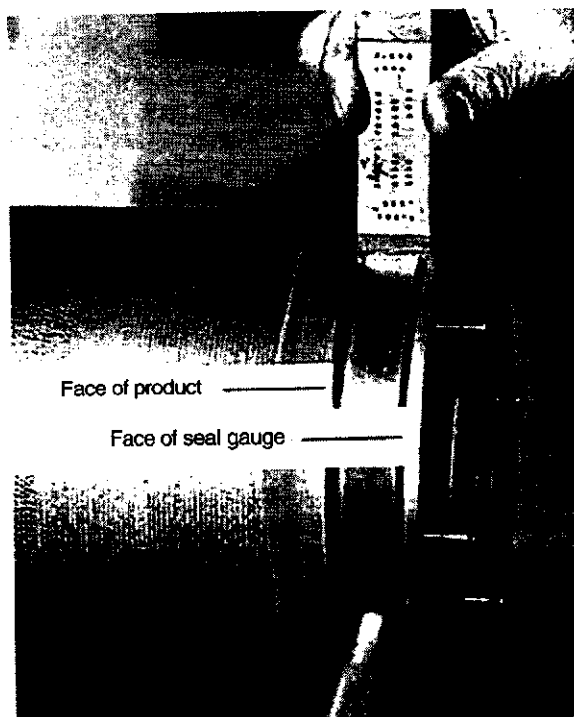
Figure 58—Extreme-Line Thread Plug Gauge Installed Hand-Tight and Seal Plug Advanced (Go-No-Go in Place for Measuring Seal Diameter)
