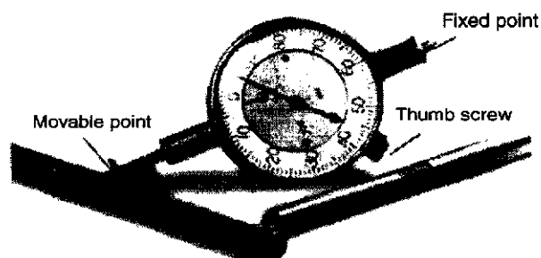
Figure 29—Internal Taper Caliper for 4 1/2-in. OD and Larger Showing Gauge Extensions
