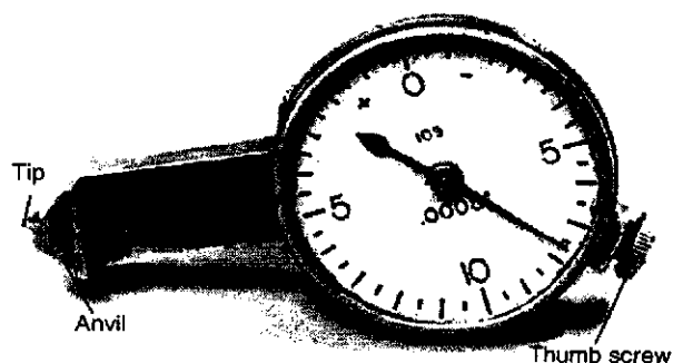
Figure 18—Balanced-Dial Type Gauge for Measuring Thread Height of Internal Threads and All External Threads
