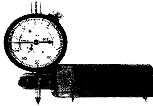
Figure 41—Buttress Thread Runout Gauge
