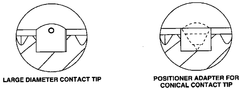
Figure 62—Detail of Alternate Acceptable Contact Tip Configurations
