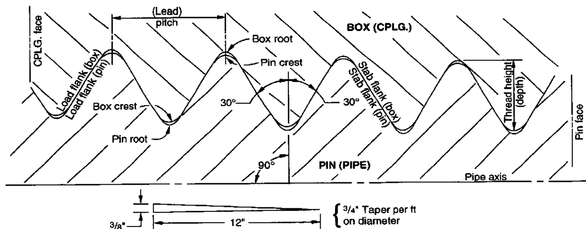
Figure 4—Round Thread Casing and Tubing Thread Configuration
