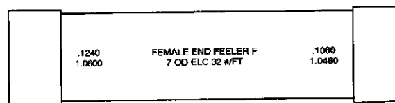
Figure 54—Go-No-Go Feeler Gauge for Extreme-Line Plug Gauge
