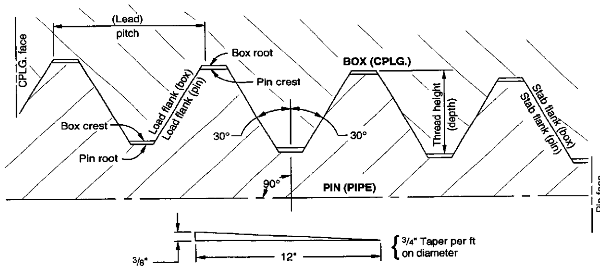
Figure 3—Line Pipe Thread Configuration
