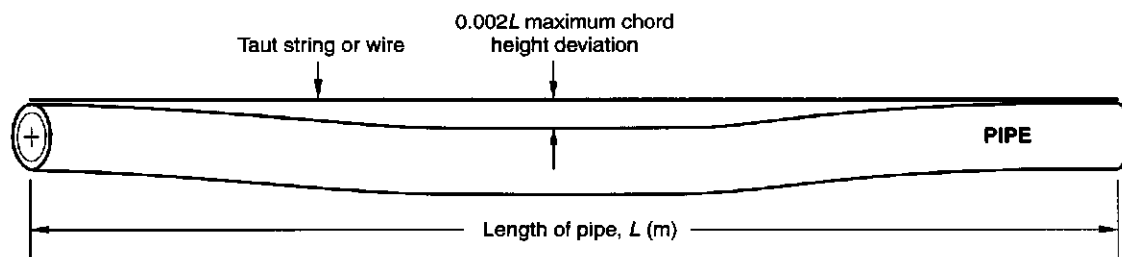
Figure 9—Measuring Full Length Straightness
