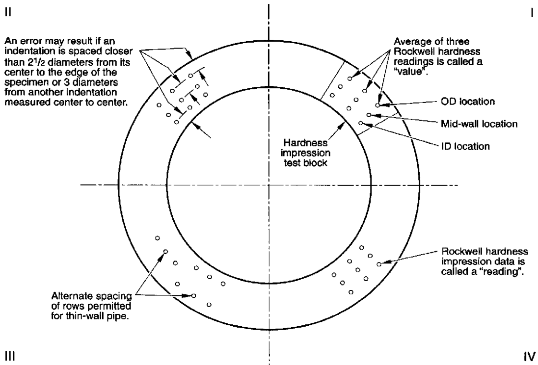
Figure 13—Through Wall Hardness Test
