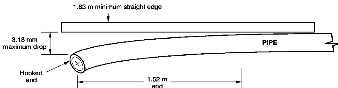
Figure 10—Measuring End Straightness
