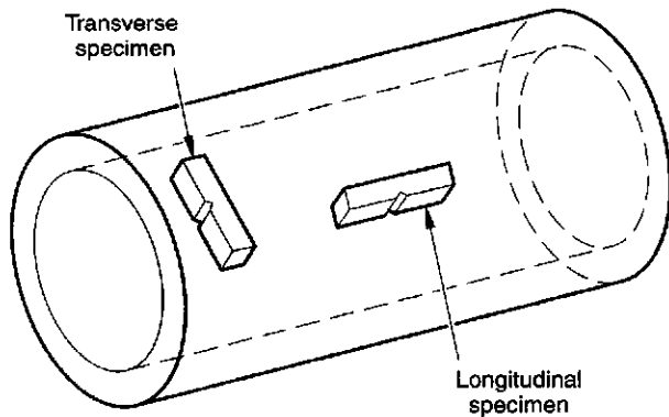
Figure 14—Impact Test Specimen Orientation
