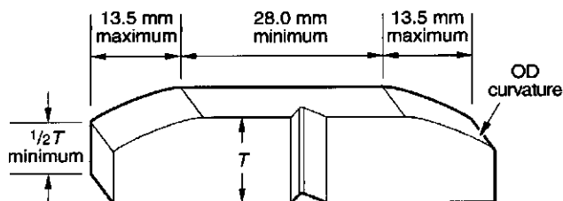
Figure B-6—Impact Test Specimen OD Curvature Allowance
