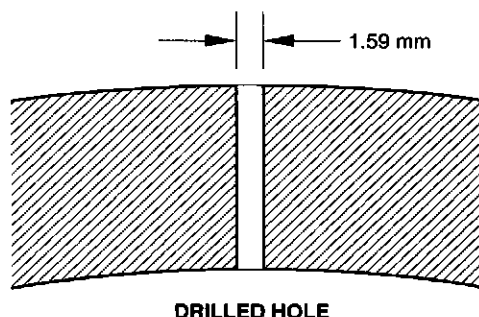
Figure B-1—Reference Standard
