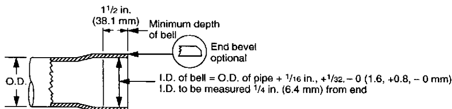
Figure 1—Belled End for Bell and Spigot Joint
