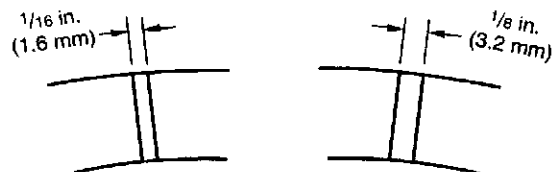
DRILLED HOLE
