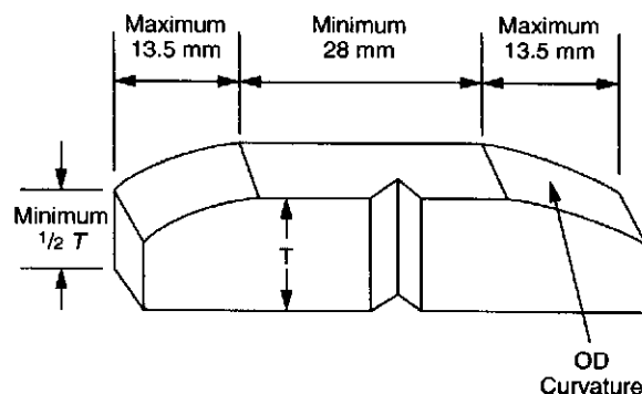
Figure F-2—Impact Test Specimen Tapered End Allowance
