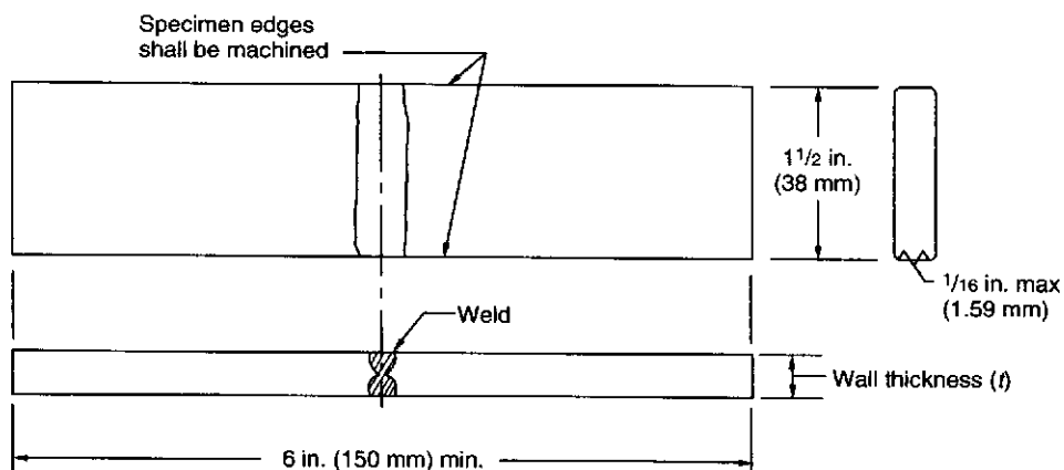
Figure C-1—Transverse Tensile Test Specimen
