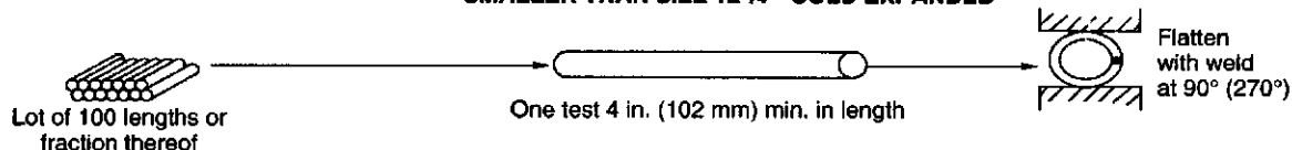
Figure 5—Flattening Tests
