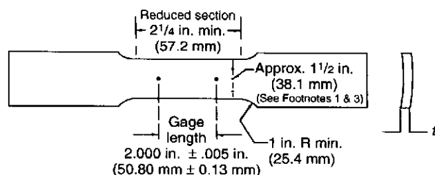
C – Strip Specimen
