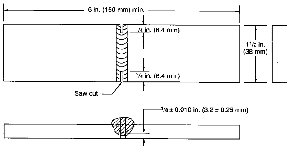
Figure C-4—Nick-Break Test Specimen
