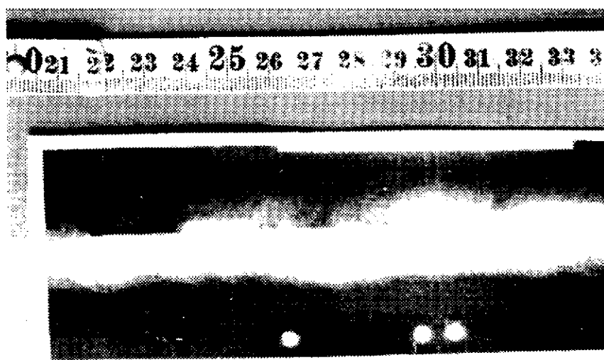
Figure 24—Incomplete Fusion
