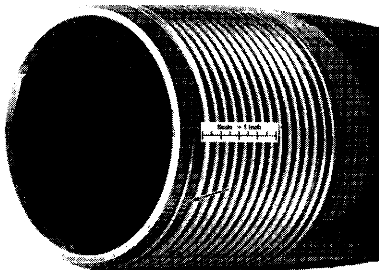
Figure 4c—Chatter on Threads & Chamfer
