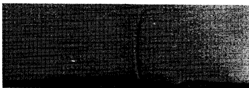
Figure 19—ERW—Hook Cracks (or Upturned Fiber Imperfections)
