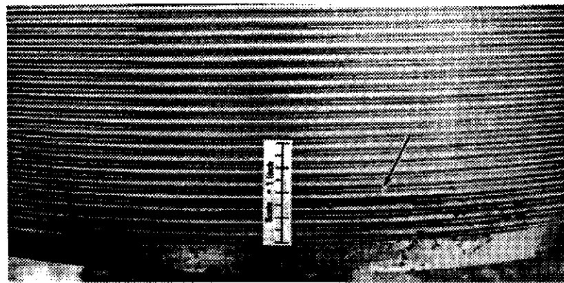
Figure 34b—Pitting, Thread Flanks & Chamfer
