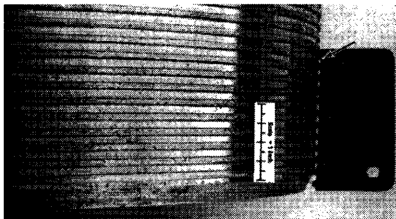
Figure 21—Improper Thread Height/Tool Marks on Crest
