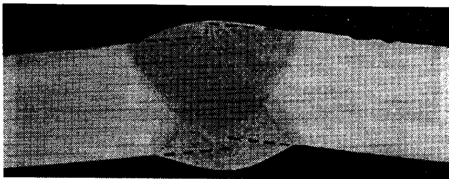
Figure 29—Offset of Plate Edges (DSA)
