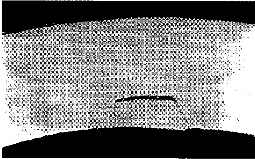
Figure 38—Rolled-In (Slug)
