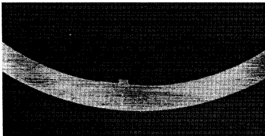
Figure 22—Inadequate Flash Trim of ERW Seam
