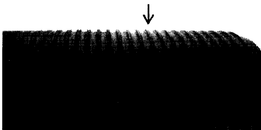
Figure 41—Shaved (or Thin) Buttress Threads
