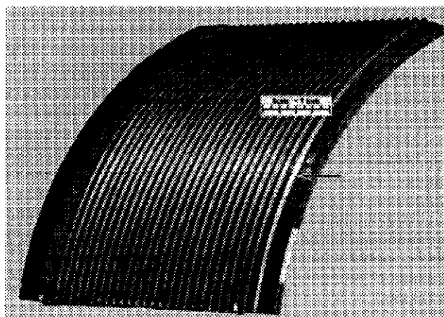
Figure 4b—Tool Chatter on Flanks
