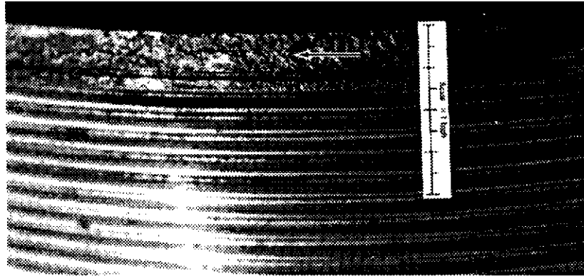
Figure 34a—Pitted Chamfer/Threads
