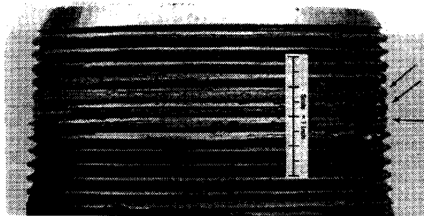
Figure 16—Galled Threads
