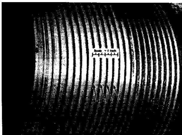
Figure 50a—Torn Threads
