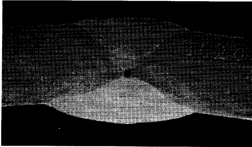
Figure 25—Incomplete Penetration (DSA)
