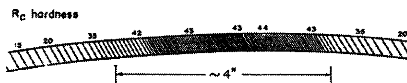
Figure 18—Hard Spot (Typical Hardness Survey)
