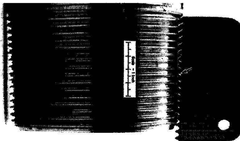
Figure 20b—Improper Thread Form (Profile Gauge)
