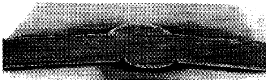
Figure 51—Undercut
