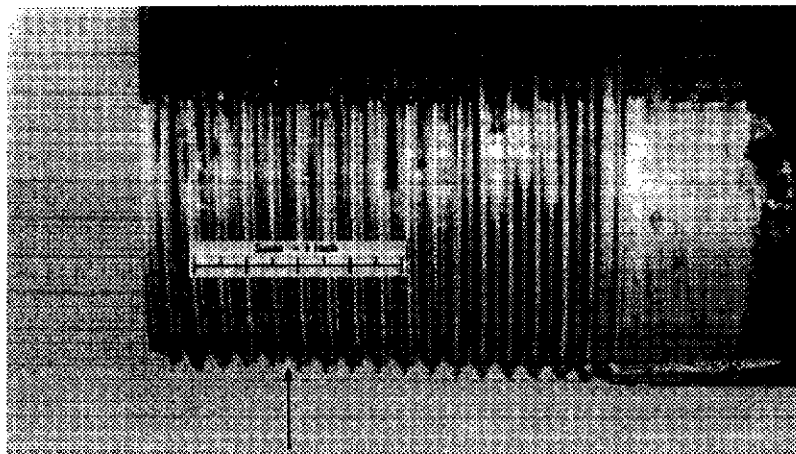
Figure 20a—Improper Thread Form
