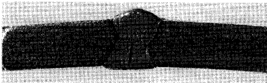
Figure 36a—Porosity-Macroetch
