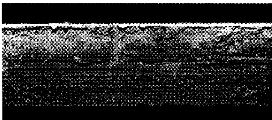
Figure 5—Cold Weld (ERW)
