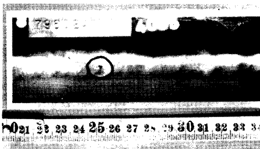
Figure 43—Slag Inclusions-Radiograph
