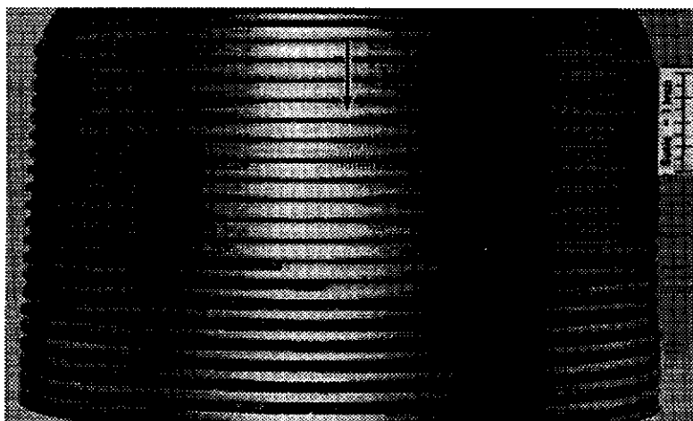
Figure 4a—Chattered Threads
