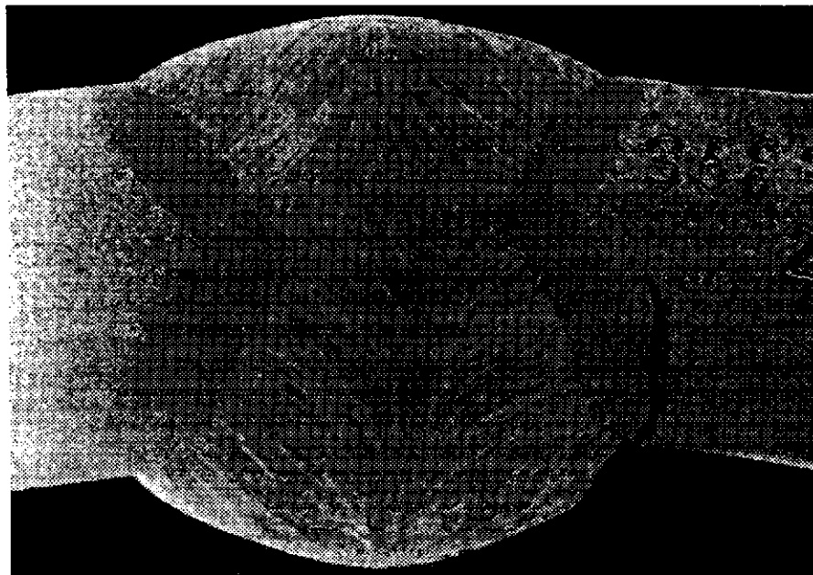
Figure 54b—Weld Area Crack
