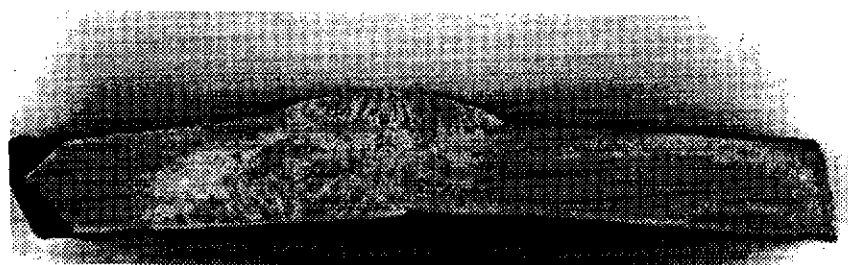
Figure 30—Out-Of-Line Weld Beads (or Off Seam)
