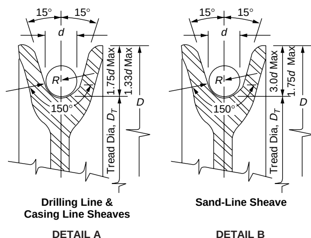
Figure 10—Sheave Grooves
