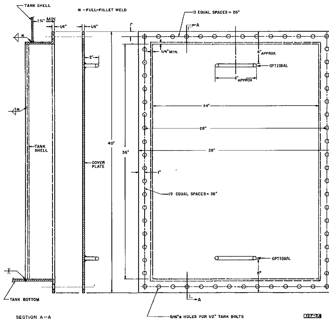
Figure 4—24-In. x 36-In. Extended-Neck Cleanout (See 3.16)
