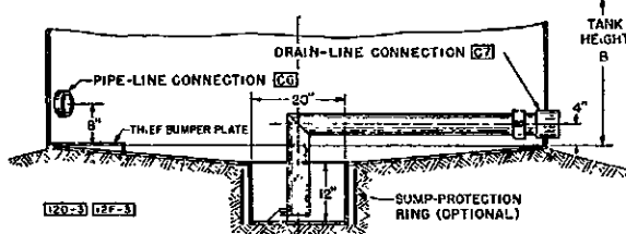
Figure 2—Type A (Unskirted) Cone Bottom
