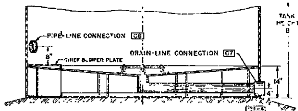
Figure 3—Type B (Skirted) Cone Bottom
