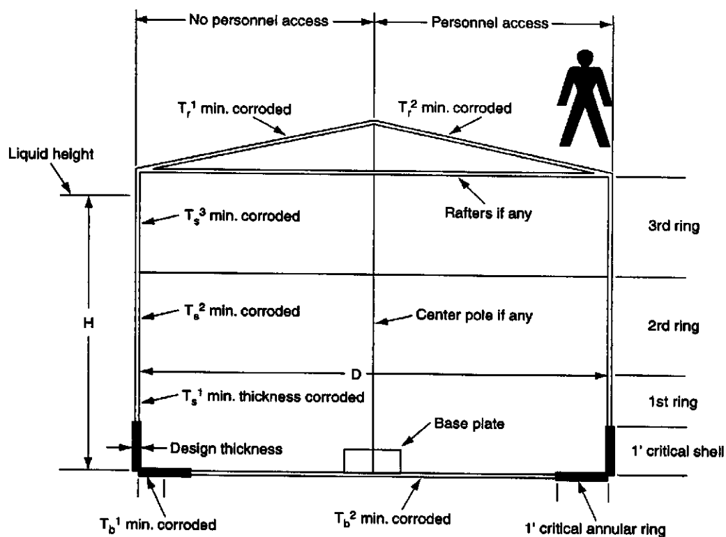
Figure 4—Corrosion Calculation Nomenclature
