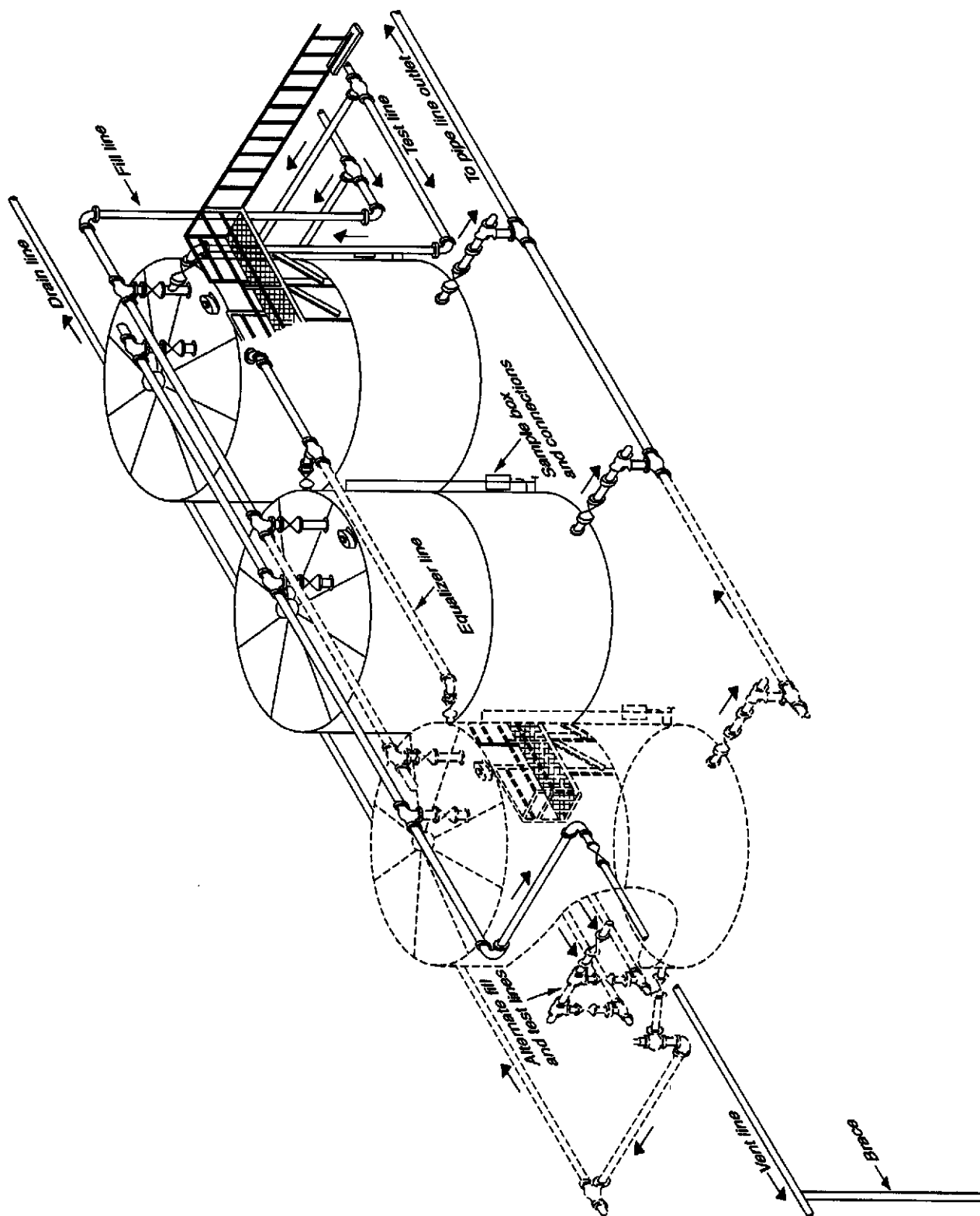
Figure 1—Example of Straight Line Tank Battery Installation and Piping Configurations
