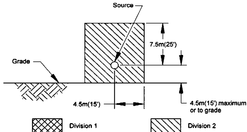
Figure 23—Adequately Ventilated Compressor Shelter With Lighter-Than-Air Gas Or Vapor Source (See Section 9.2.2.1)
