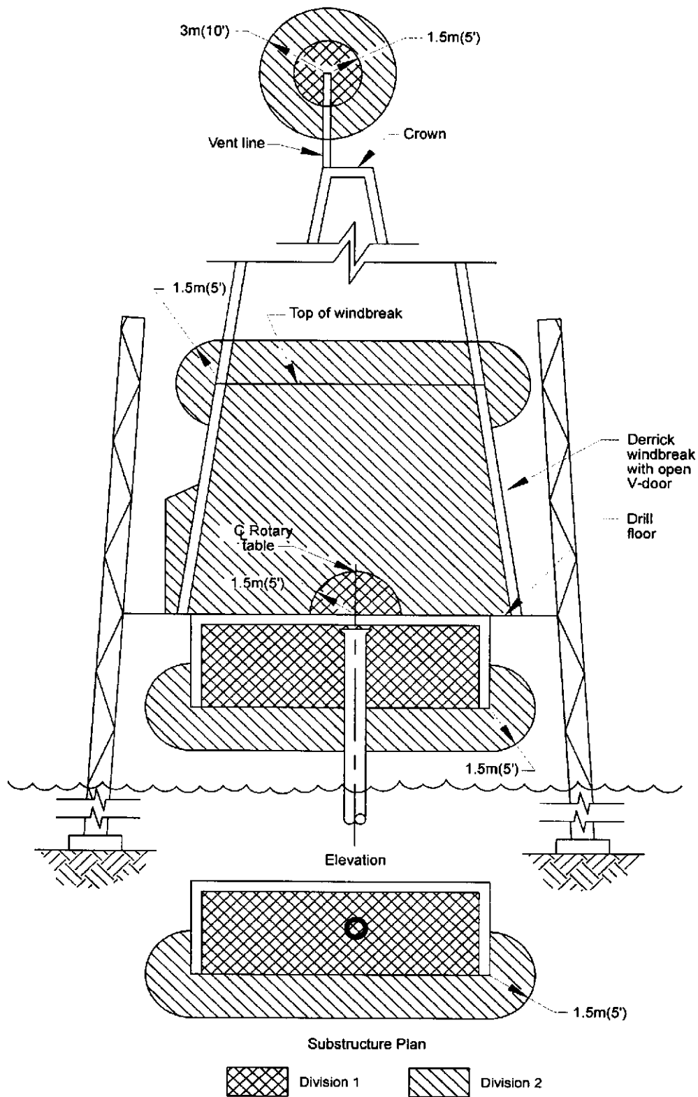
Figure 72—Drilling Rig Semi-enclosed Substructure and Semi-Enclosed Derrick (See Section 11.8.3)
