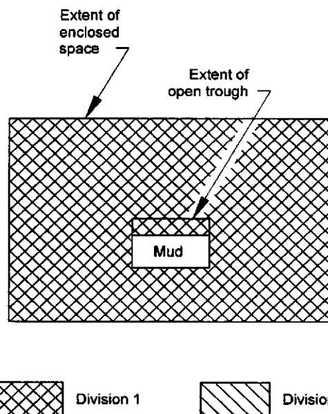
Figure 80—Open Mud Trough in Enclosed Space With Adequate Ventilation Before Degasser (See Section 11.11.1)
