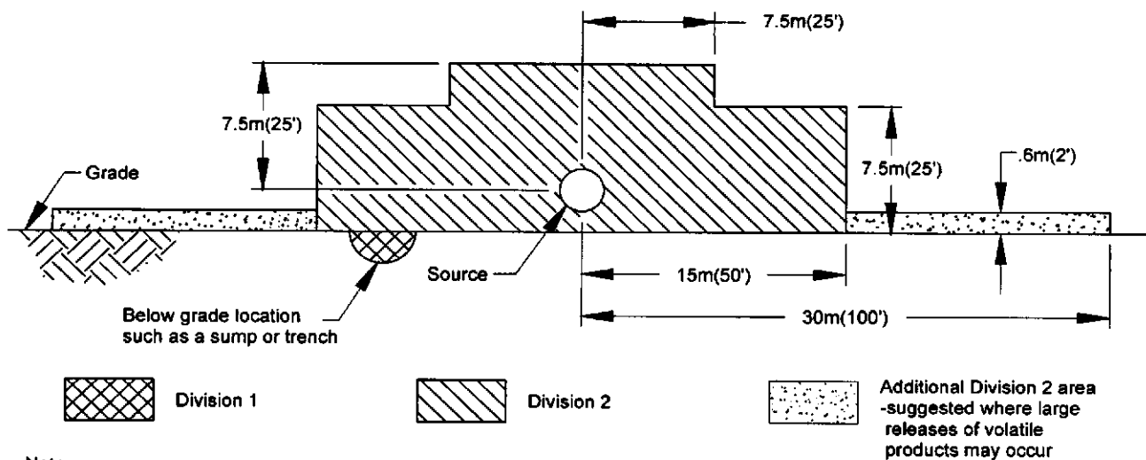
Figure 20—Adequately Ventilated Process Location With Heavier-Than-Air Gas Or Vapor Source Located Near Grade (See Section 9.2.1.1)
