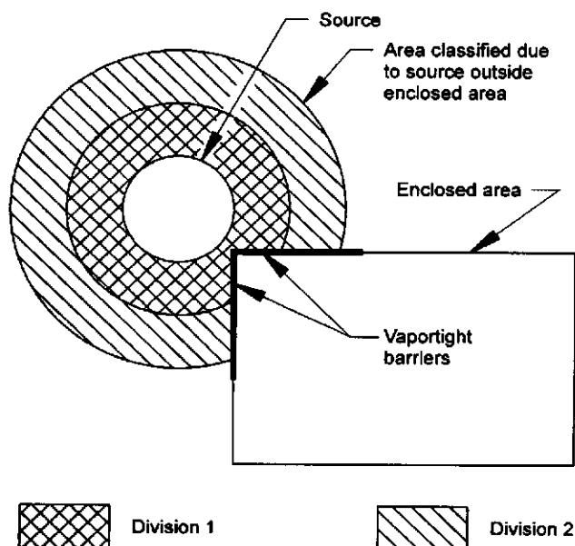
Figure 3—Enclosed Area Adjacent to a Classified Area (See Section 6.4.2)
