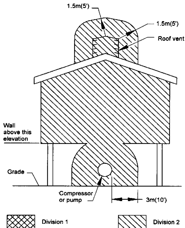
Figure 52—Compressor Or Pump In An Adequately Ventilated Nonenclosed Area (See Section 10.9.1)
