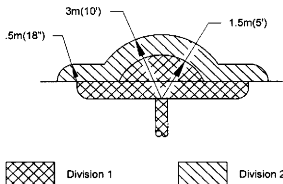
Figure 62—Type 4 Open Drain System in Nonenclosed Area (See Sections 10.13.4.1, 10.13.4.2, 10.13.4.3, and 10.13.4.4)
