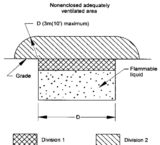
Figure 57—Open Sump in Nonenclosed Adequately Ventilated Area (See Sections 10.12.1, 10.12.2, and 10.13 Note 4)
