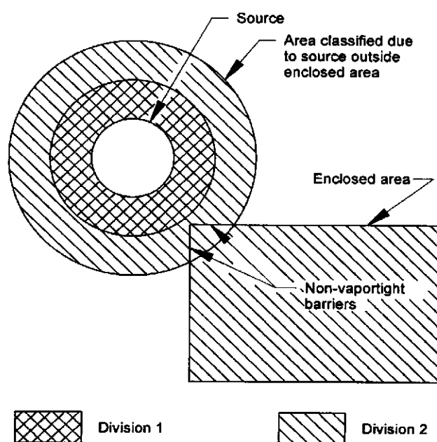
Figure 5—Enclosed Area Adjacent to a Classified Area (See Section 6.4.3)
