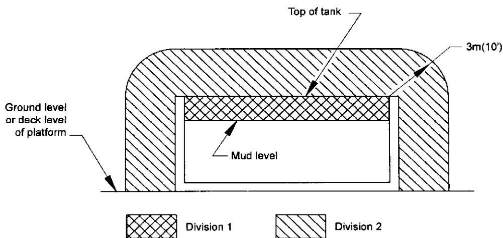
Figure 33—Mud Tank in a Nonenclosed Adequately Ventilated Area (See Sections 10.4.2.1, 10.4.3.1, and 10.12.2)
