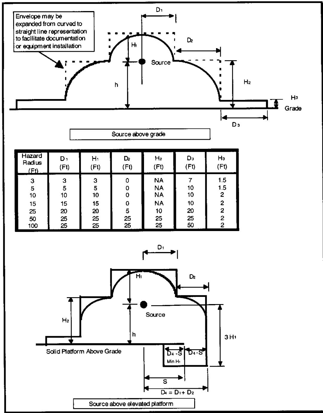
Figure D-3—Adequately Ventilated Process Area With Heavier-Than-Air Gas or Vapor Source Located Near or Above Grade
