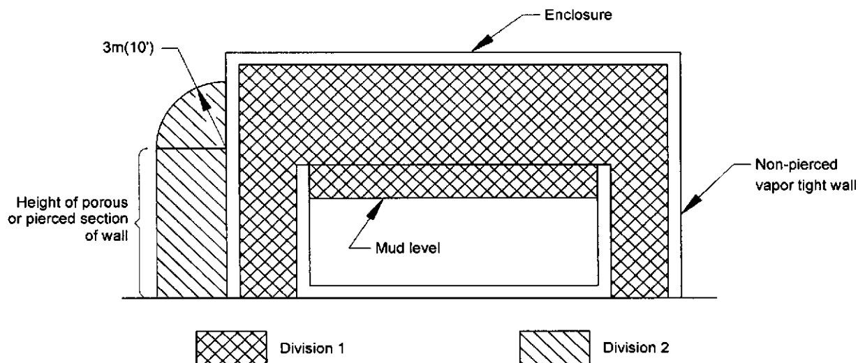
Figure 34—Mud Tank in an Inadequately Ventilated Area (See Sections 10.4.2.3, 10.4.3.3, and 10.12.3)
