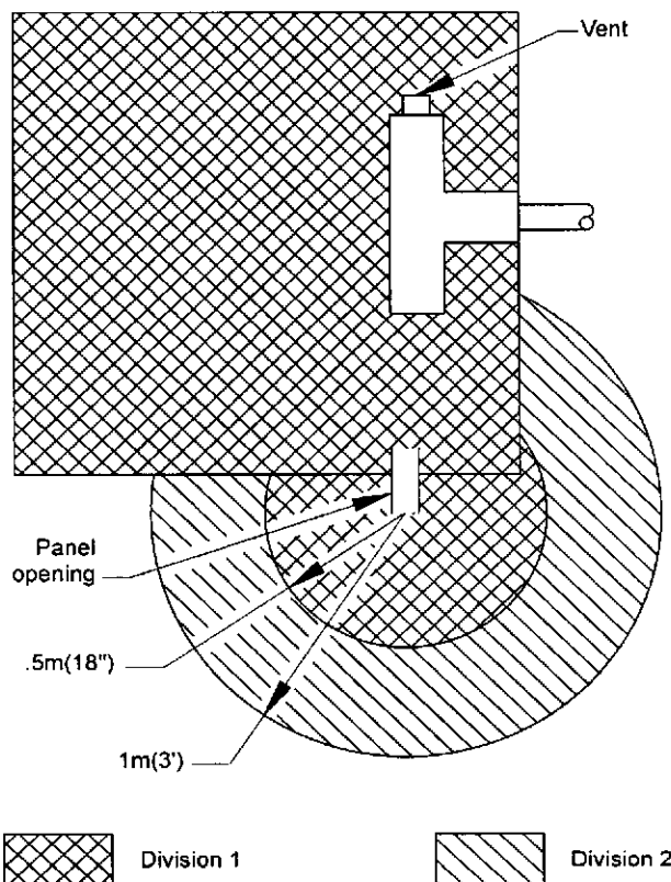
Figure 64—Control Panel With Flammable Gas Vented to the Inside of the Enclosure (See Section 10.16.3)
