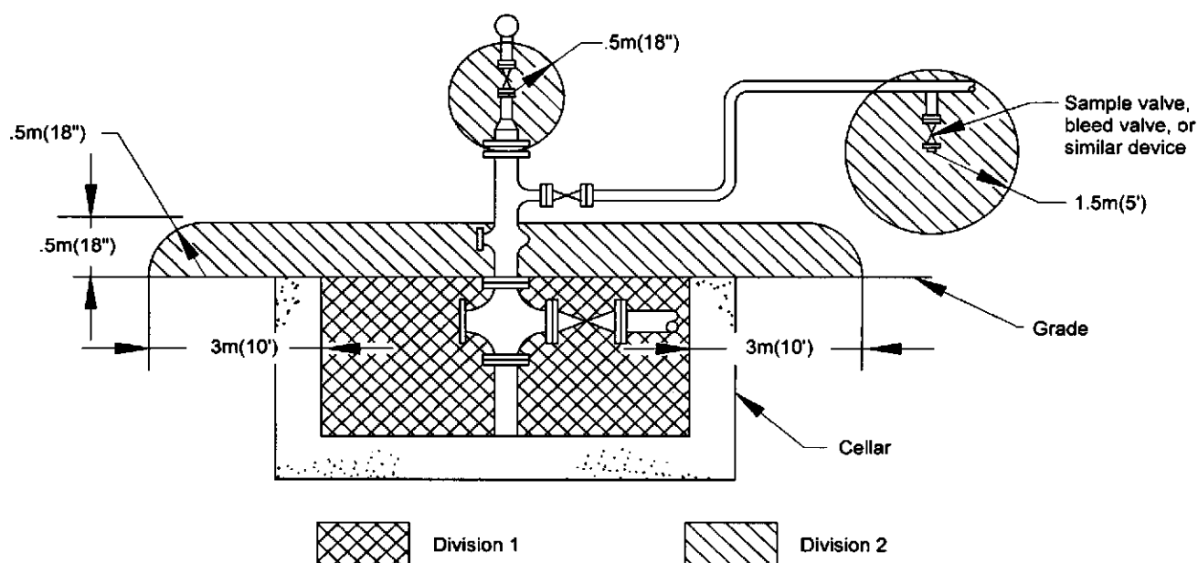
Figure 40—Flowing Well in a Nonenclosed Adequately Ventilated Area With an Inadequately Ventilated Cellar or Below Grade Sump (See Sections 10.5.1.2 and 10.15.3.2)
