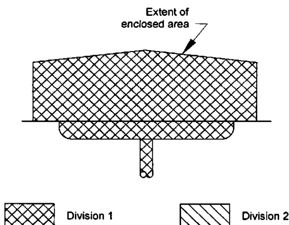
Figure 63—Type 4 Open Drain System in Enclosed Area (See Sections 10.13.4.5 and 10.13.4.6)
