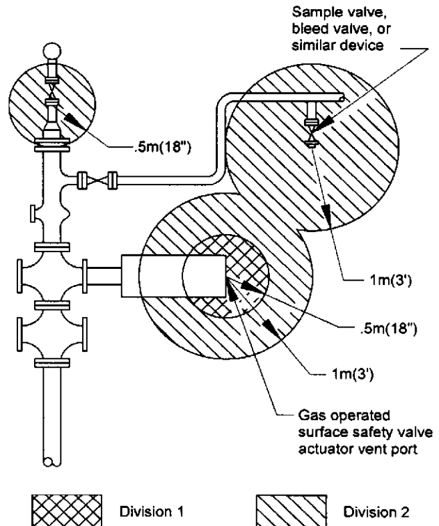
Figure 39—Flowing Well in a Nonenclosed Adequately Ventilated Area and Without a Cellar or Below Grade Sump (See Sections 10.5.1.1 And 10.15.3.2)
