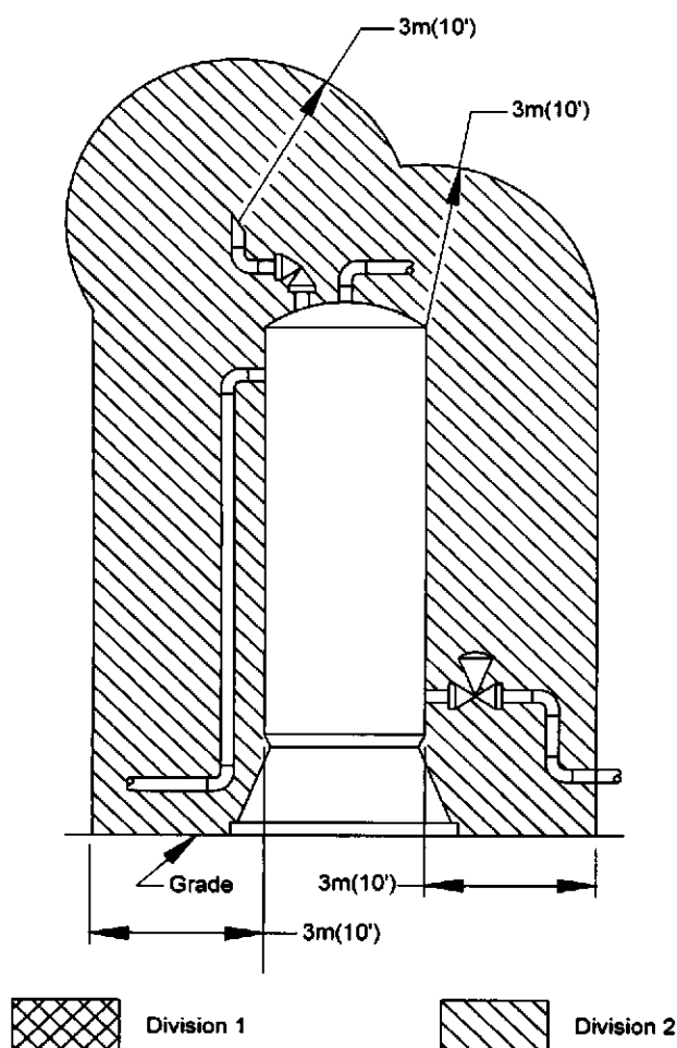
Figure 48—Hydrocarbon Pressure Vessel or Protected Fired Vessel in a Nonenclosed Adequately Ventilated Area (See Sections 10.6.3.1, 10.6.5.1, and 10.6.7.1)
