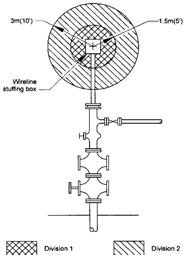
Figure 42—Nonenclosed Adequately Ventilated Well on Which Wireline Work Is Being Performed (See Sections 10.5.1.7.1 and 10.5.1.7.2)
