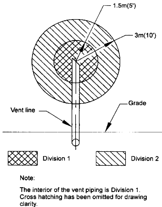
Figure 38—Degasser Vent in Nonenclosed Adequately Ventilated Area (See Section 10.4.7.4)
