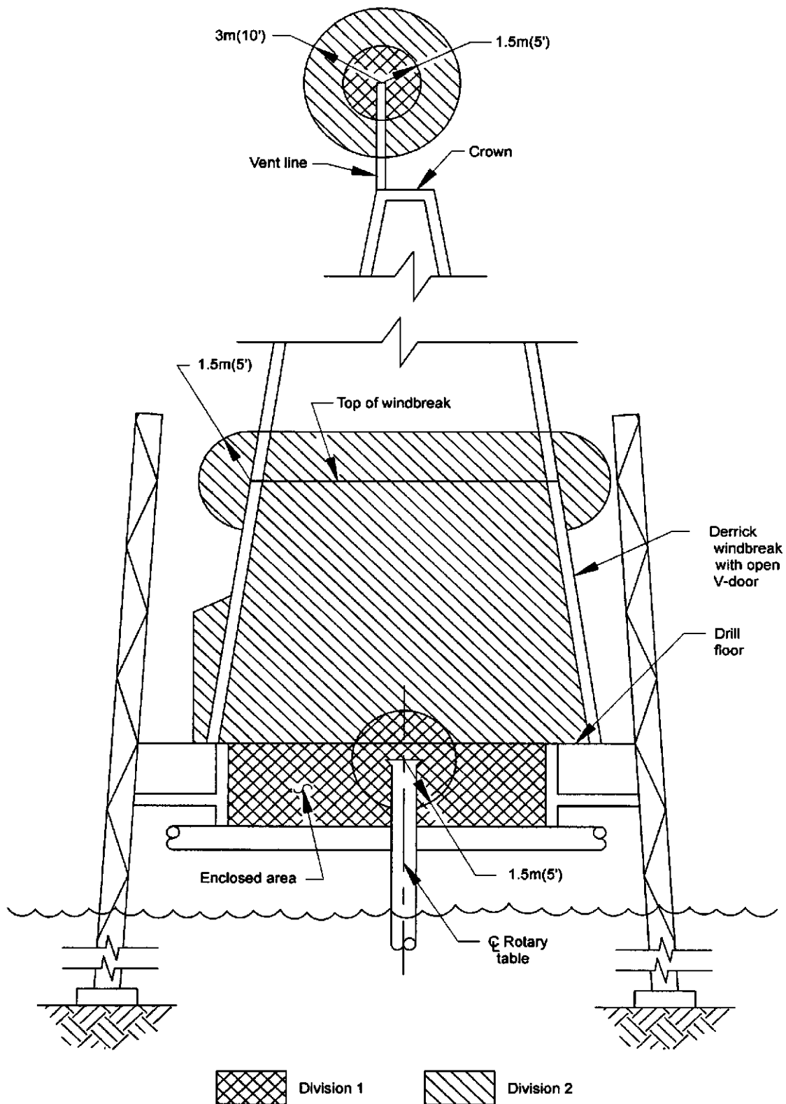
Figure 71—Drilling Rig With Total Containment Substructure and Semi-Enclosed Derrick (See Section 11.8.2)
