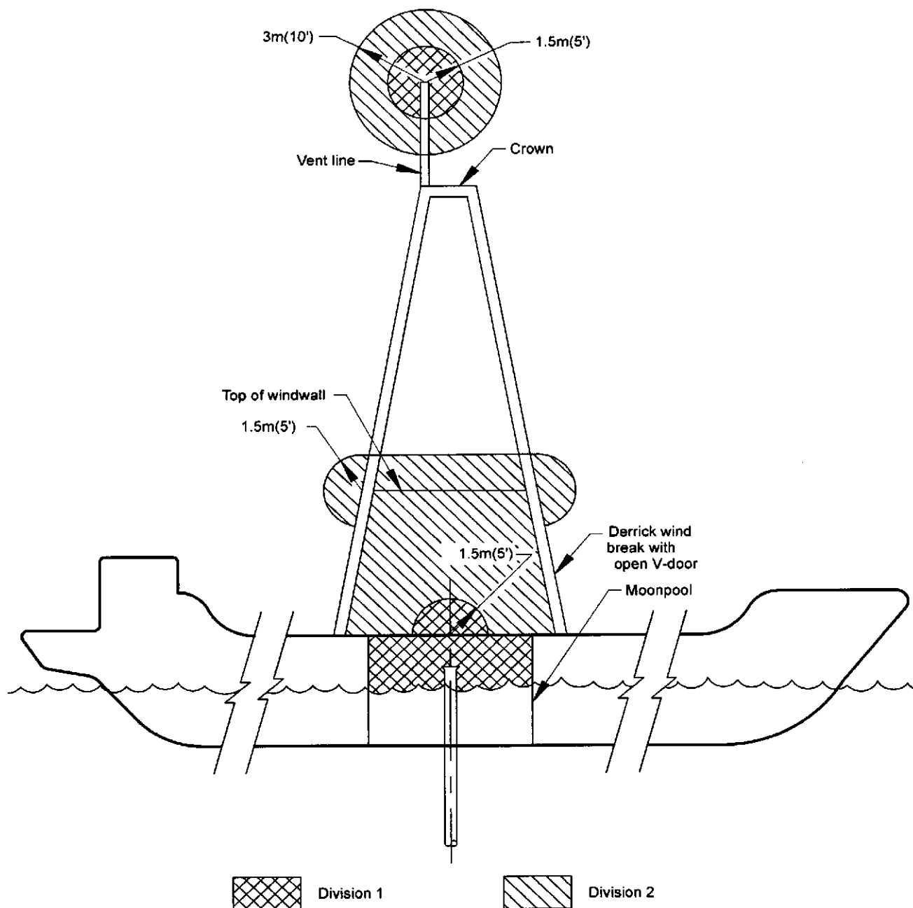
Figure 73—Drilling Rig Enclosed Moonpool and Semi-Enclosed Derrick (See Section 11.8.4)
