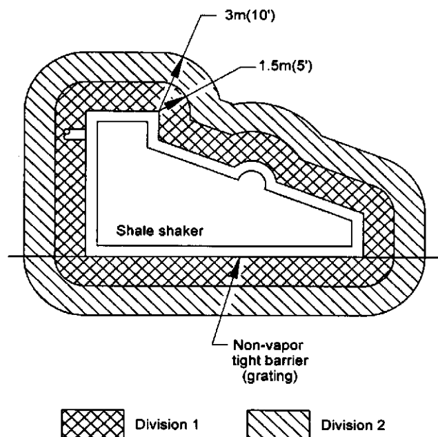
Figure 35—Shale Shaker in a Nonenclosed Adequately Ventilated Area (See Section 10.4.5.1)
