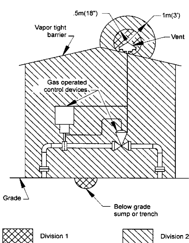
Figure 55—Flammable Gas-Operated Instruments in an Adequately Ventilated Enclosed Area With All Devices Vented to the Outside (See Section 10.11.2.2) Note: For Vents, See Section 8.2.3.2
