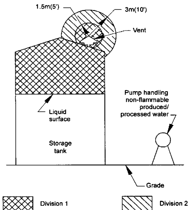
Figure 50—Flammable Gas-Blanketed and Produced Water-handling Equipment in a Nonenclosed Adequately Ventilated Area (See Sections 10.8 and 10.12.4)
