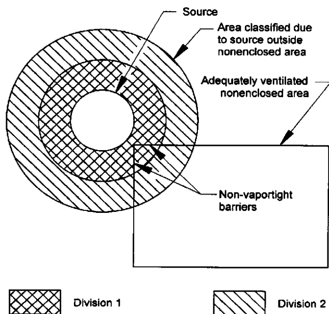
Figure 2—Adequately Ventilated Nonenclosed Area Adjacent to a Classified Area (See Section 6.4.1)
