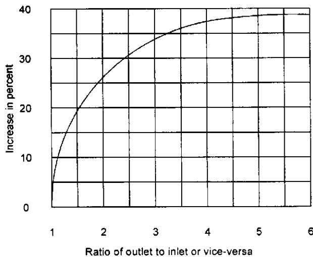
Figure 1—Increase in Flow Caused by Excess of One Opening Over Another (See Section 6.3.2.4.6)
