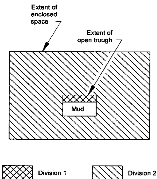
Figure 80—Open Mud Trough in Enclosed Space With Adequate Ventilation Before Degasser (See Section 11.11.1)
