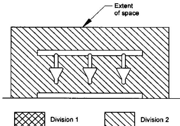
Figure 85—Desander or Desilter in Enclosed or Semi-Enclosed Space With Adequate Ventilation (See Section 11.14.1)
