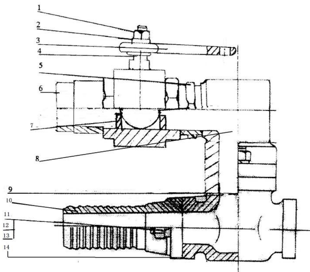
图 7 Figure 7 三通总成 B250-06-00 Tee installation
